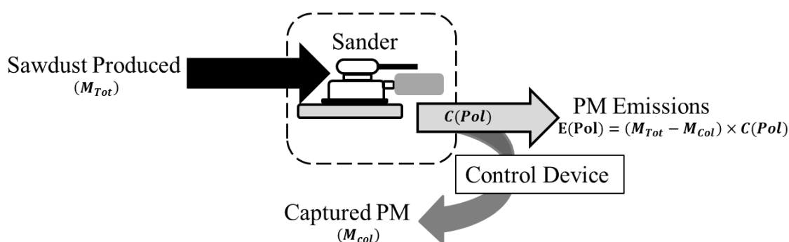
Figure 26-2. Woodworking Control Volume
