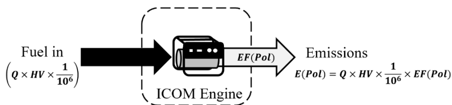
Figure 3-3. Stationary ICOM Control Volume - Fuel Consumption Method
