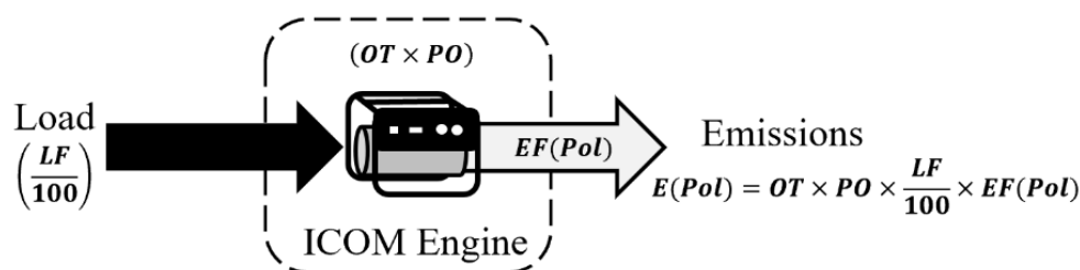
Figure 3-4. Stationary ICOM Control Volume – Load Factor Method
