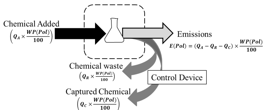
Figure 13-2. General Chemical Use Control Volume
