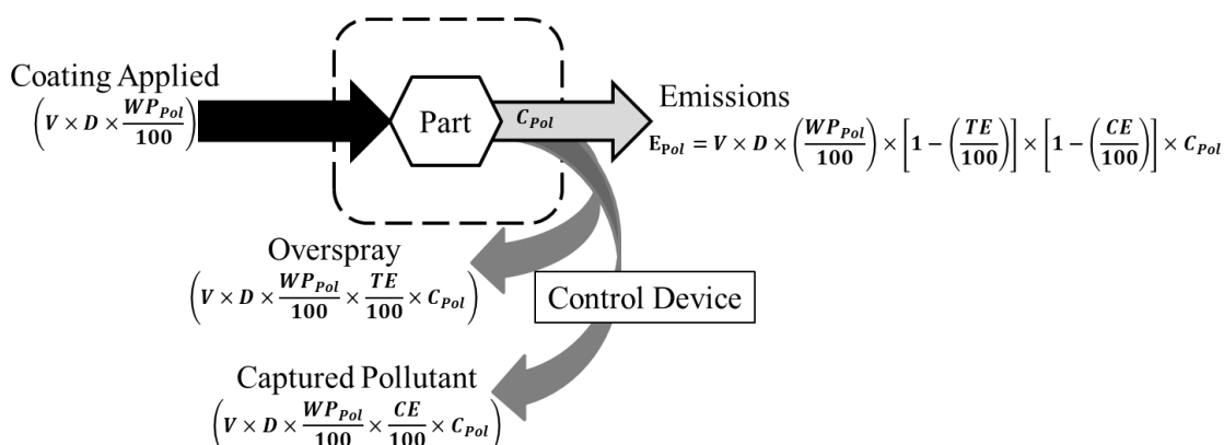
Figure 22-3. Surface Coatings Control Volume – Mass Balance Method for Particulate Matter and Inorganic HAPs
