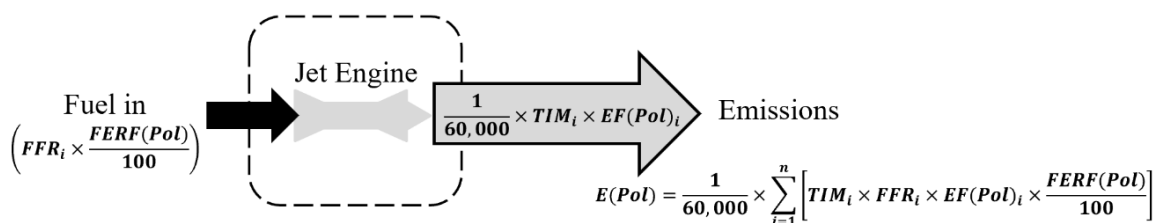
Figure 4-2. Aircraft Engine Testing Control Volume
