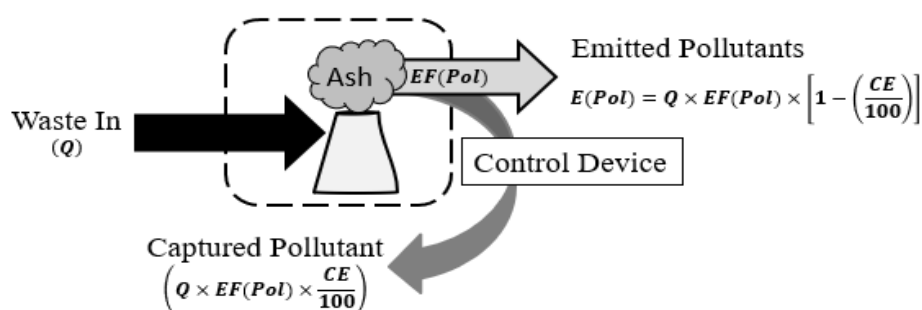
Figure 14-2. Incinerator Use Control Volume
