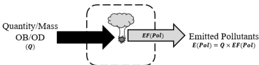
Figure 16-2. OB/OD Control Volume - Without Donor Charge
