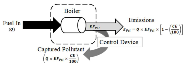
Figure 2-2. External Combustion Control Volume
