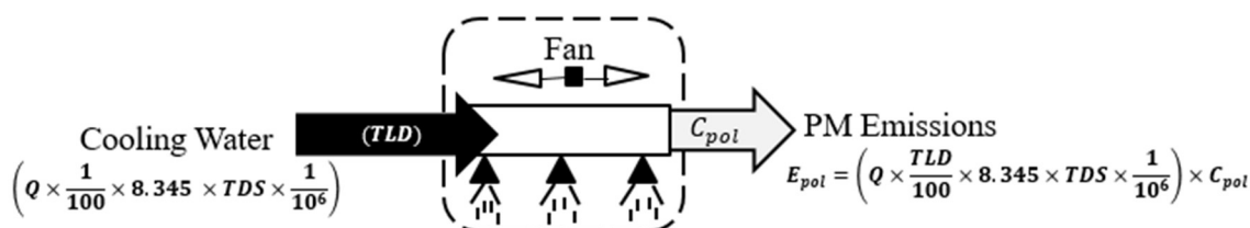
Figure 25-2. Wet Cooling Towers Control Volume
