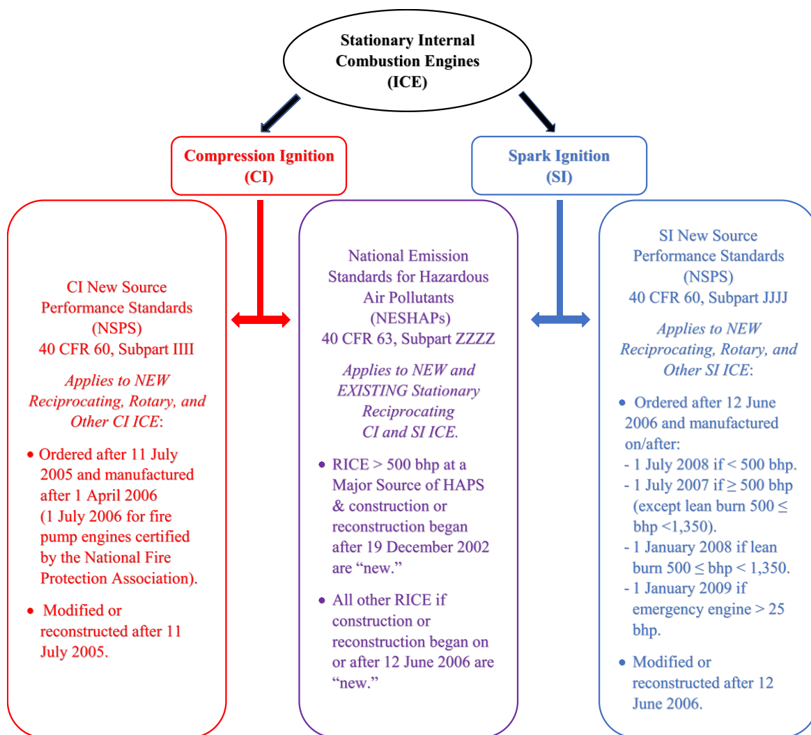
Figure 2-1. Stationary Engine Rule Flowchart
